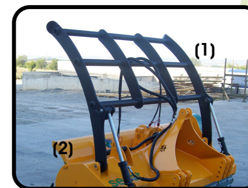
▶ Pushing frame (1) ▶ Hydraulic rear hood (2)
