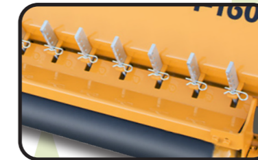
▶ Rear tine retainers
