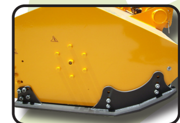
▶ Front adjustable skid shoes
