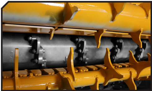
3 lines of counter knives screwed
