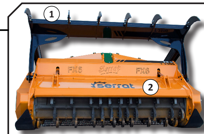
Swinging hammers
